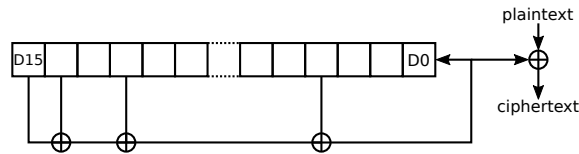
Fig. 4.2: 16-bit LFSR taps
