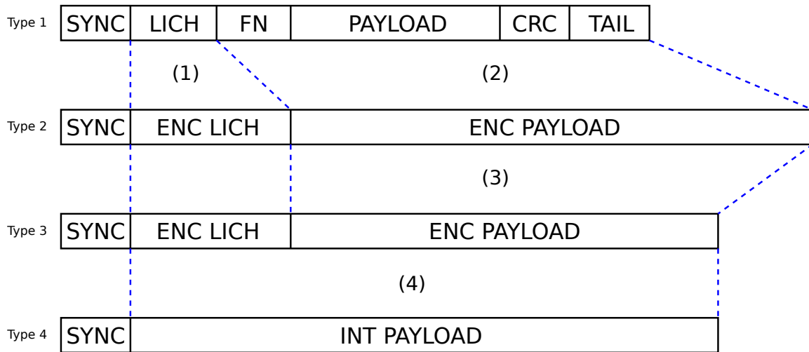
Fig. 2.3: ECC stages of subsequent frames
