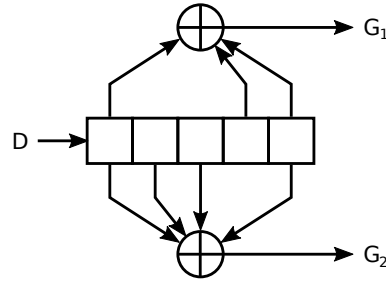
Fig. 2.4: Convolutional coder diagram
