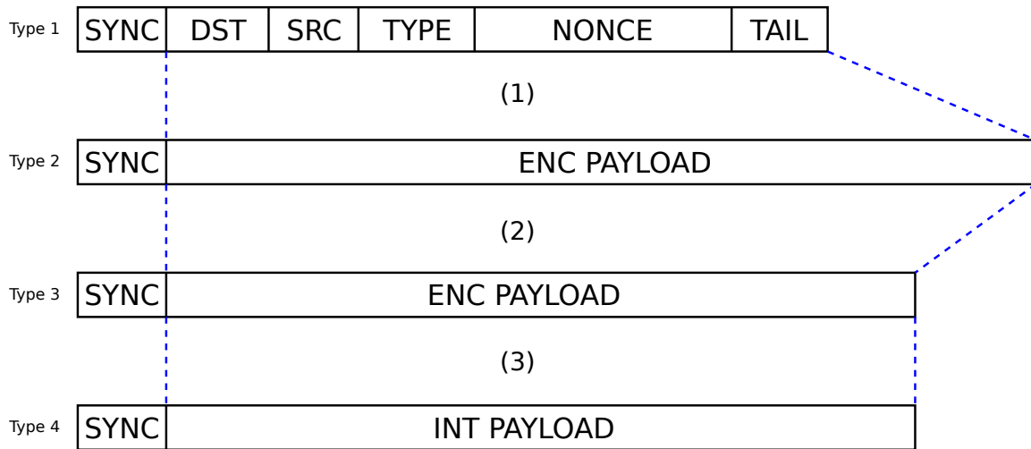
Fig. 2.2: ECC stages for the link setup frame
