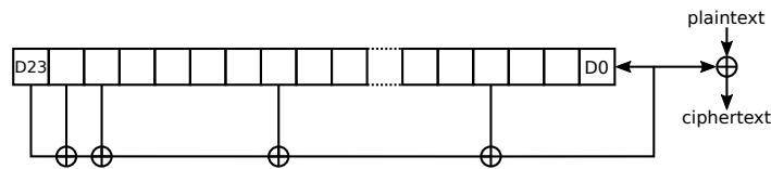
Fig. 4.3: 24-bit LFSR taps
