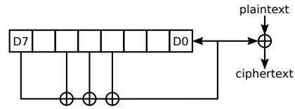
Fig. 4.1: 8-bit LFSR taps
